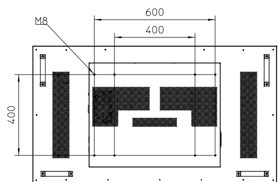
rear view1
