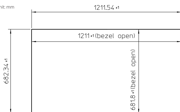
front view1
