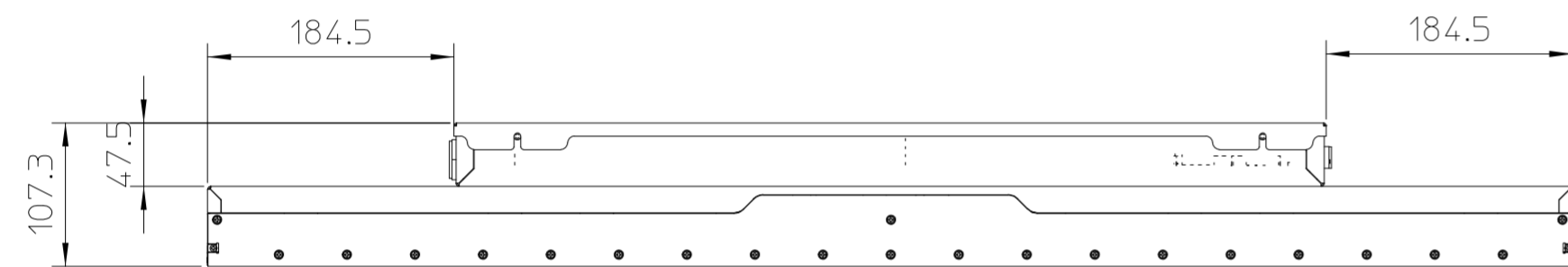
plan view1
